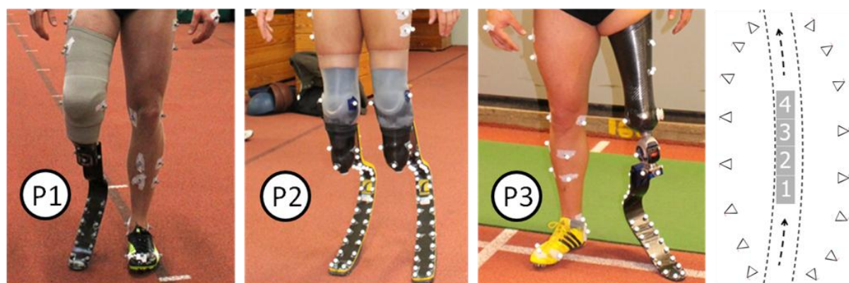
Figure 1: Lower limbs of the amputee athletes (left: P1 right side below knee; middle left: P2 bilateral below knee; middle right: P3 left side knee exarticul) and the technical set up (right) including cameras, force plates, ground marking and running direction is shown.
