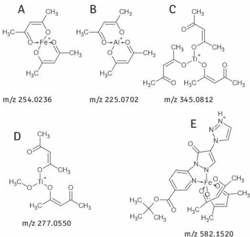
Figure 2: Volatile metal complexes with acetyl acetone (A-D) and IOX4 adduct with \text{Fe}(\text{AcAc})^{2+} (E)
