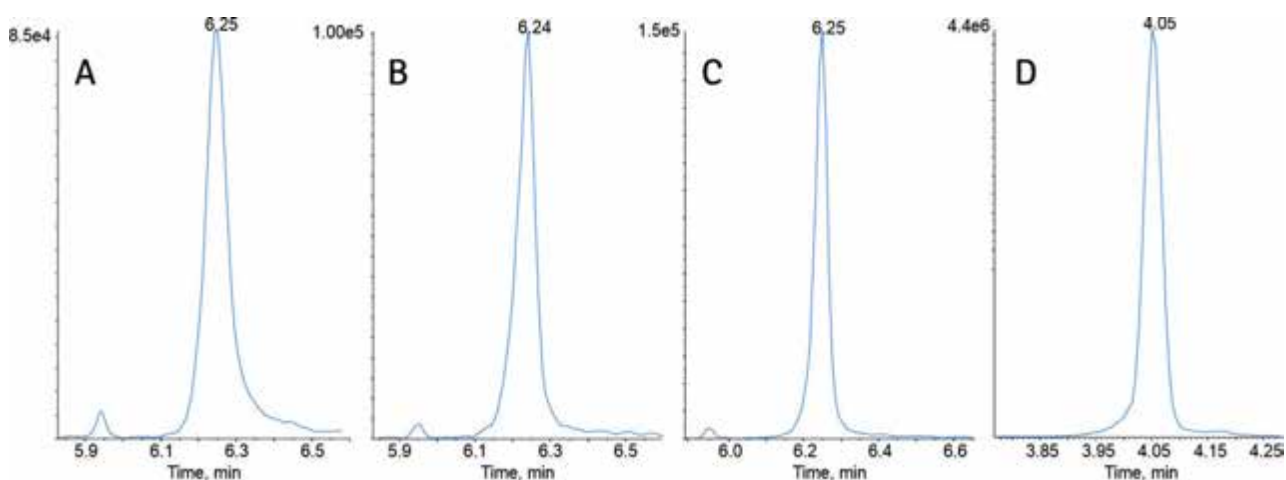
Figure 3: Peak shape of IOX4 (A-C) and molidustat (D) on Premier HSS T3 column (both at 2 ng/mL, 329 > 273 and 315 > 207 , ESI+, respectively), A: brand new column, B-C: precolumn replaced, first injection (B) and 96 th injection (C)
