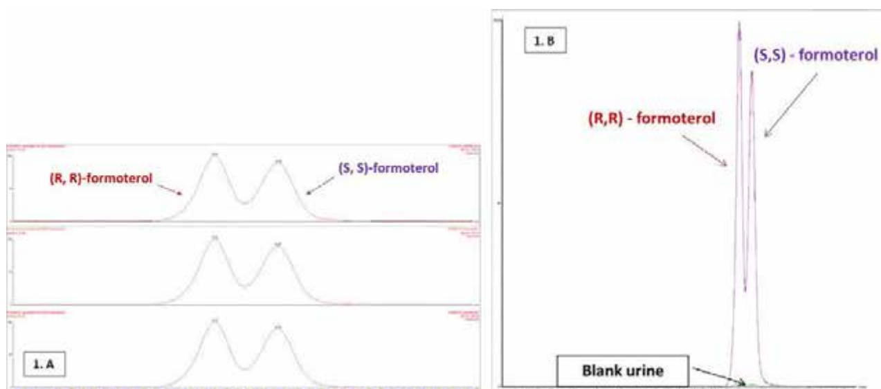
Figure 1. A Chromatogram of formoterol enantiomers in QC sample (10 ng/mL); B Exemplary UPLC-MS/MS chromatogram of real case sample of formoterol in urine overlaying a blank urine sample
