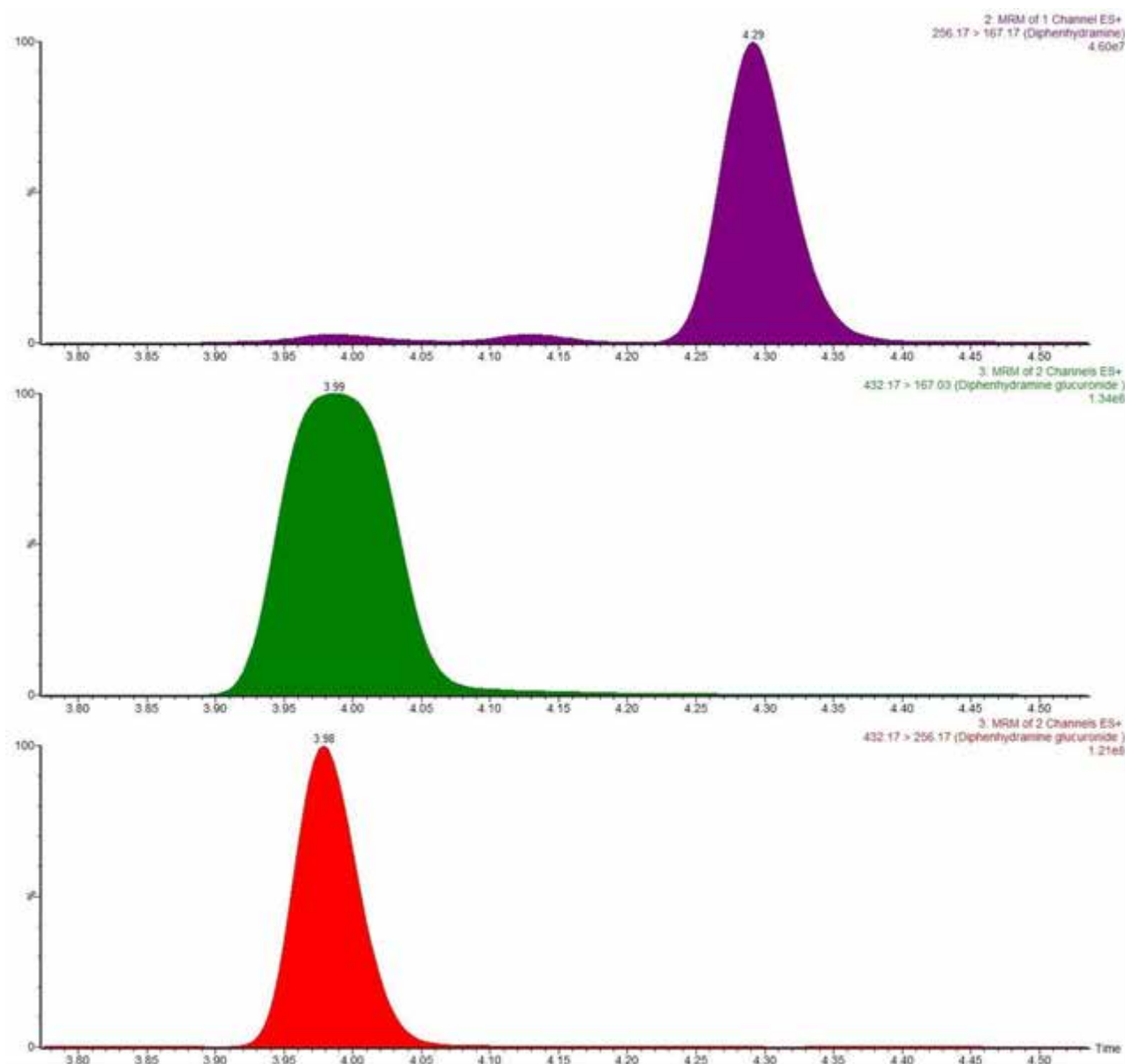
Figure 3. Chromatograms of an athlete urine from the Initial Testing Procedure prepared with the DaS method
