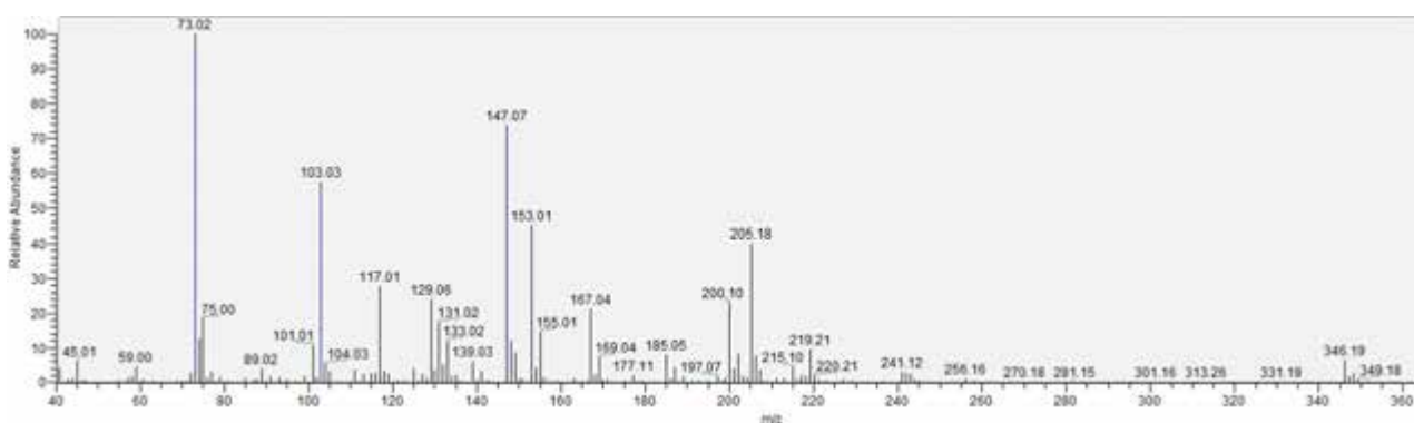
Figure 3. Chlorphenesin carbamate spectrum
