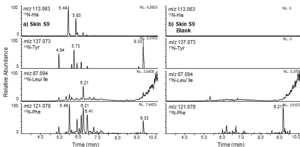
Figure 1. AIF chromatogram of the extracted ion traces corresponding to the most abundant ^{15}\text{N} -labelled immonium ions, showing the metabolites obtained after incubation of ^{15}\text{N} -hGH in skin S9 mix (a) in comparison to the respective substrate blank (b)
