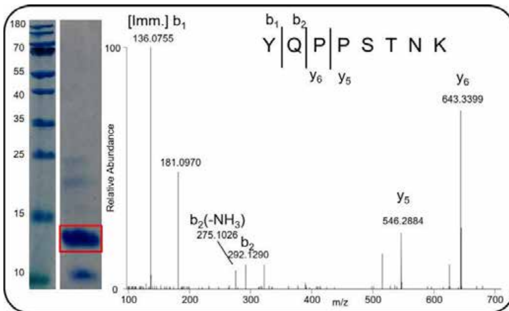
Figure 3: MS 2 -product ion mass spectrum @ ce 30 of trypsin-digested SDS-PAGE-spot (ca. 13 kDa, red frame). Precursor of tryptic MGF-fragment: m/z 934
