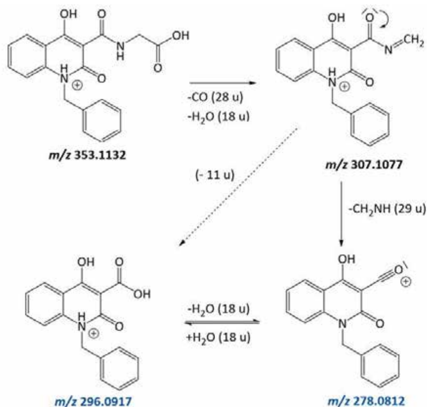
Figure 2. Proposed dissociation pathway of the protonated IOX-2 molecule including a reversible gas-phase addition of water in ion trap mass spectrometers
