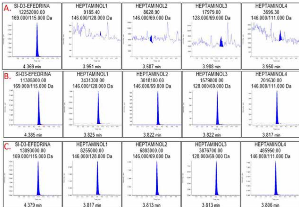
Figure 3. Chromatograms for: A. Negative control, B. Positive control 20 ng/mL, C. Heptaminol standard in H 2 O 40 ng/mL
