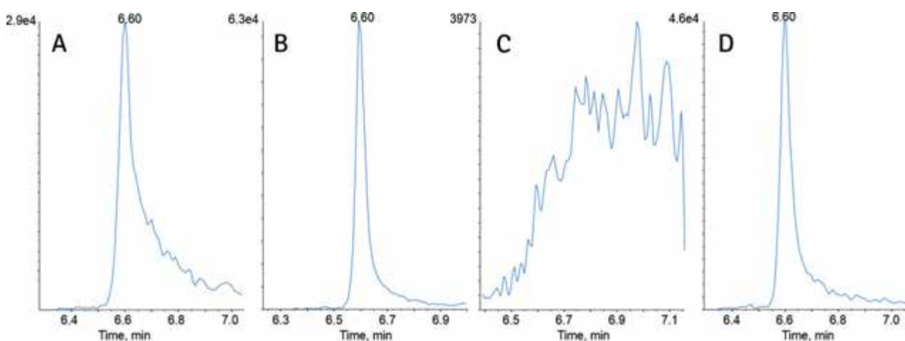
Figure 1. Peak shape of IOX4 (2 ng/mL, 329 > 273, ESI+) on Cortecs T3 column, A-B: well-used precolumn & column, first injection (A), 96 th injection (B), C-D: precolumn replaced, first injection (C) and 96 th injection (D).
