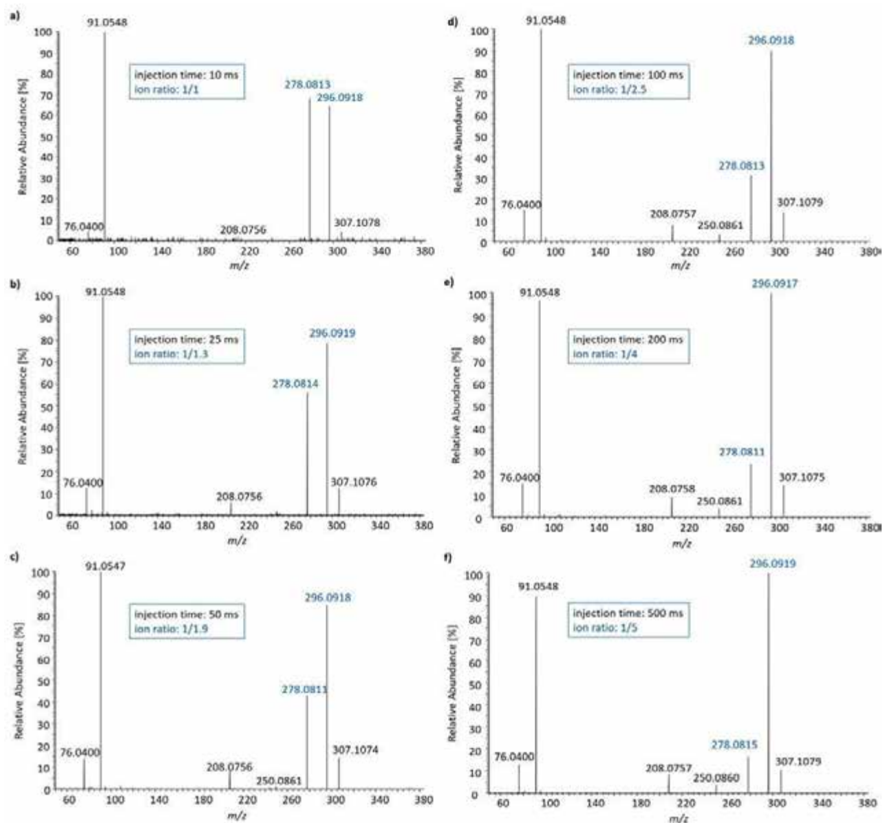
Figure 1. Comparison of IOX-2 ( m/z 353.1132) product ion mass spectra using a constant AGC target set to 5e^6 and a variable maximum injection time of a) 10 ms, b) 25 ms, c) 50 ms, d) 100 ms, e) 200 ms and f) 500 ms, demonstrating a significant correlation between the injection time and the shift of the product ion ratio between m/z 278 and m/z 296 towards the water adduct
