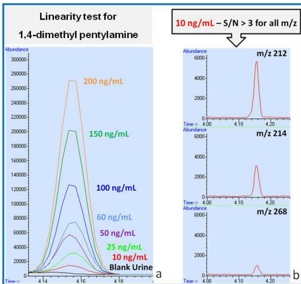
Figure 4. Total ion chromatogram obtained for the linearity test (a) and extraction of the three ions selected at the level of 10 ng/mL (b), of 1,4-dimethyl pentylamine
