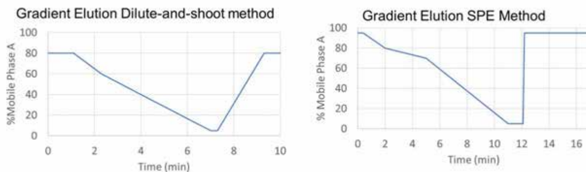
Figure 1. Chromatographic conditions – gradient elution
