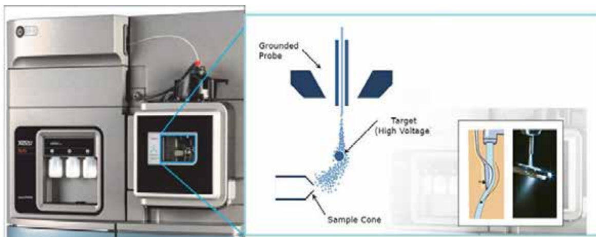
Figure 2. Unispray source shown on the Xevo TQ-XS [Source: Waters]
