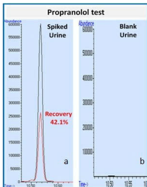
Figure 2. Total ion chromatogram for the spiked urines (a) and the blank urine (b) obtained for propranolol test
