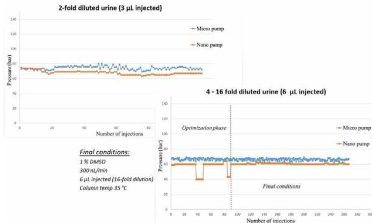
Figure 1. Pressure monitoring of the online automatic filtration setup
