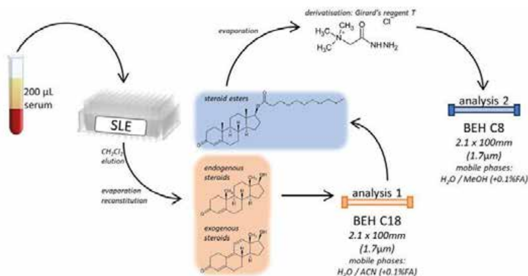
Figure 1. Schematic illustration of the sample preparation and analytical workflow for the analysis of endogenous and exogenous steroids as well as steroid esters from one aliquot of 200 µL serum
