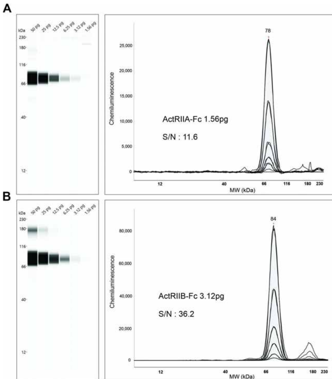
Figure 1. Detection limits for ActRIIA-Fc and ActRIIB-Fc reference preparations. Samples were initially prepared to contain 50 pg of each molecule in 4 \mu L of PBS 1X/BSA 0.0025 %. Serial dilutions were performed down to 1.56 pg for each molecule, and samples were heat denatured following the addition of 1 \mu L of PS 5X buffer. Amounts are based on the absolute quantity in 5 \mu L of sample loaded on the wells of the pre-filled plates and analyzed by Wes automated capillary electrophoresis immunoassay. Detection limit, presented on the right panel is based on the lowest amount for which a peak with a ratio S/N >10 is obtained. A) Detection limit for ActRIIA-Fc. B) Detection limit for ActRIIB-Fc.
