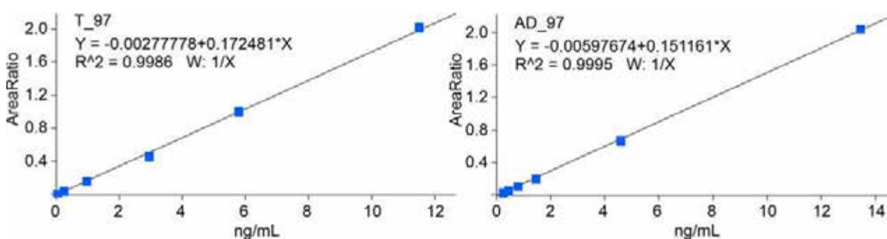
Figure 1. Calibration curves for testosterone and androstenedione
