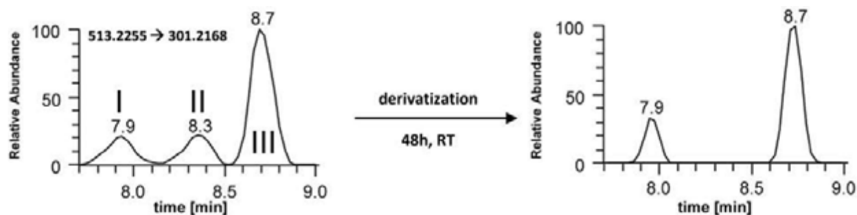
Figure 1. Results of derivatization experiment with tritylchloride; XIC, m/z 513.2255 \rightarrow 301.2168 (35eV), ESI-, 5 ppm mass tolerance
