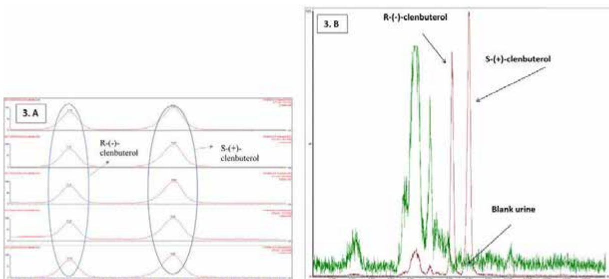
Figure 3. A Chromatogram of clenbuterol enantiomers (0.2 ng/mL); B Exemplary UPLC-MS/MS chromatogram of real case sample of clenbuterol in urine overlaying a blank urine sample
