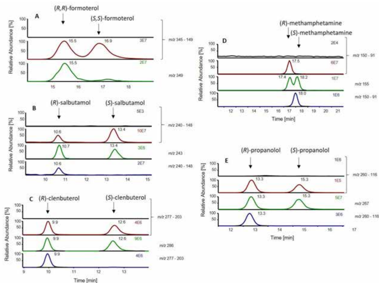
Figure 1. Extracted ion chromatograms with diagnostic precursor-product ion pairs for the target analytes (MS/MS experiments) and precursor ion (full MS) for related ISTDs showing the separation of target analytes in urine sample extracts containing: formoterol (A), salbutamol (B), clenbuterol (C), methamphetamine (D), and propranolol (E). Blank urine specimens are shown in black, authentic urine samples containing the target analytes in red, related ISTDs in green, and the enantiopure reference standards (when available) in blue. Except for the methamphetamine enantiomers, baseline separation was accomplished.
