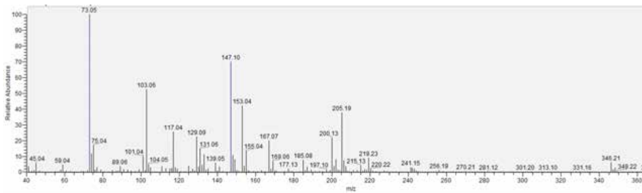
Figure 2. Chlorphenesin spectrum
