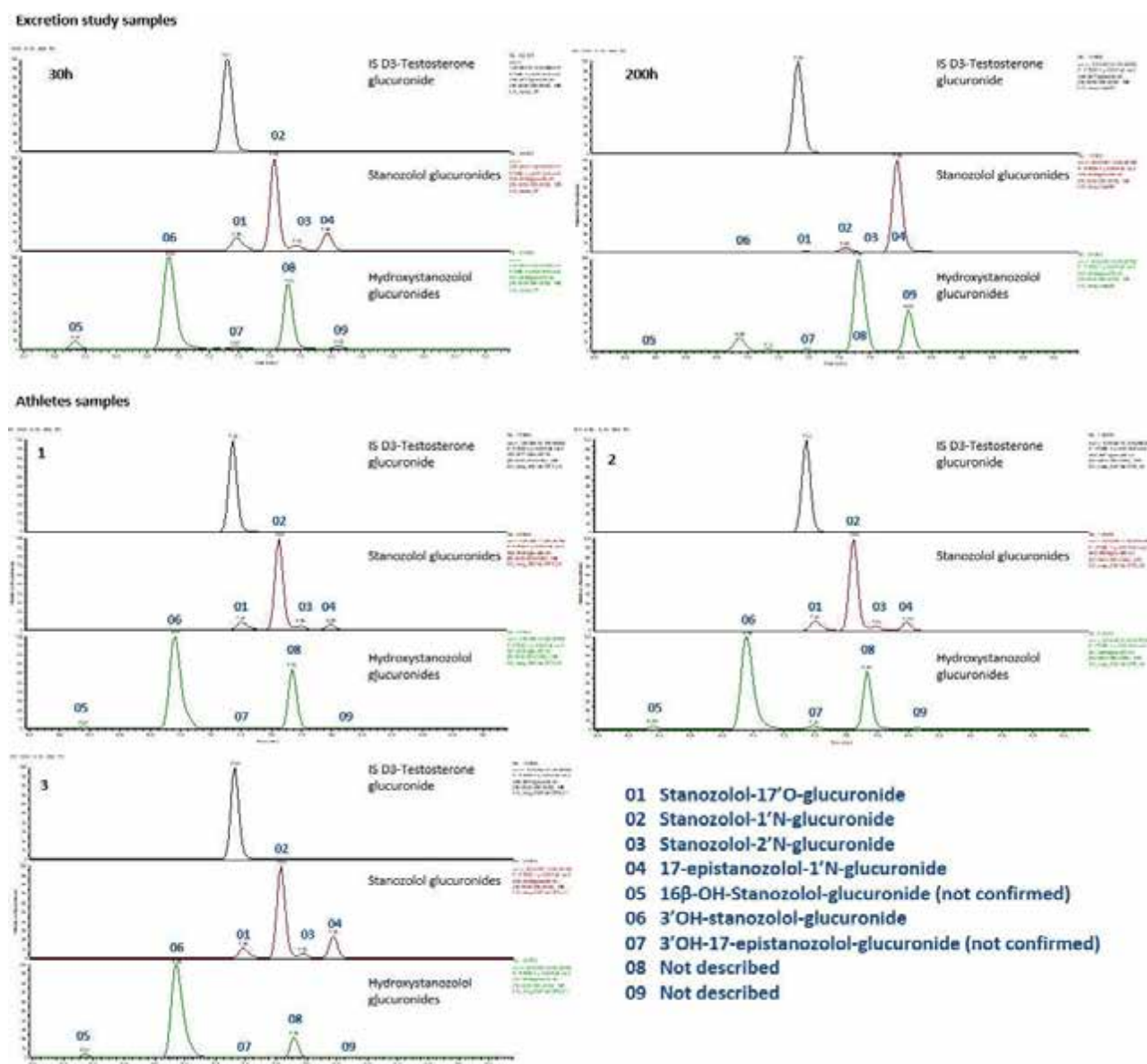
Figure 1. Online-SPE-LC-HRMS results; Above, XICs of two exemplary samples from the elimination study and below, three athlete's samples; For all samples the internal standard d3-testosterone glucuronide at ion transition 468.2671->109.0652 (CE = 35 eV), stanozolol glucuronides at ion transition 505.2908->329.2584 (CE = 60 eV) and hydroxystanozololglucuronides at ion transition 521.2858->345.2536 (CE = 60 eV) are shown
