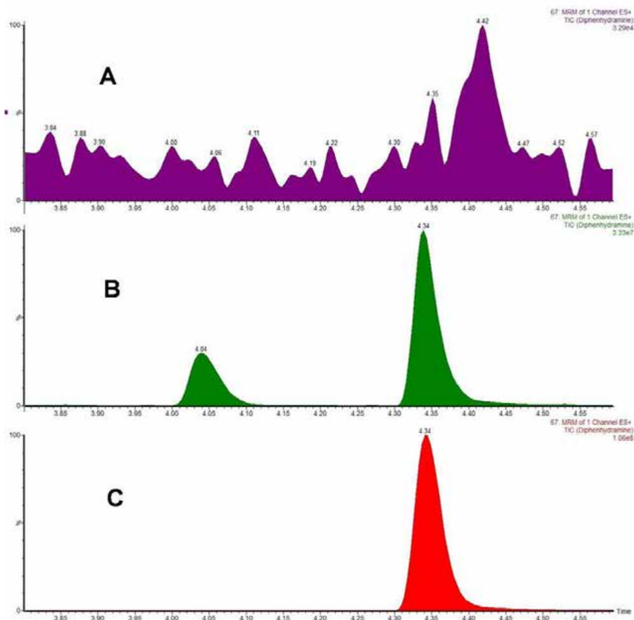
Figure 1. Chromatograms of diphenhydramine (TIC) from Initial Testing Procedure. A. Blank urine; B. Athlete`s sample and C. QC sample of diphenhydramine (25 ng/mL)
